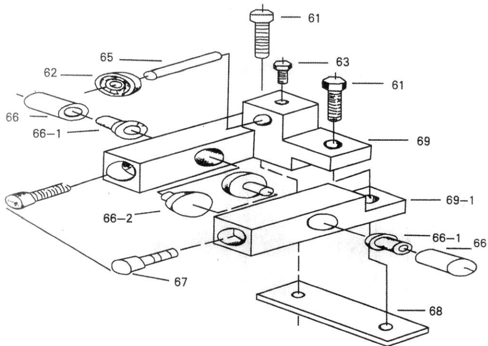
Lower saw blade guide
